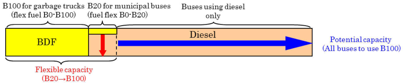
Figure 2 Potential and flexible capacities of BDF distribution system
