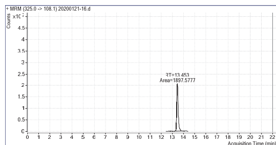
STD/0.001ng
