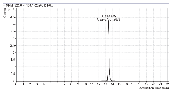
STD/0.02ng
